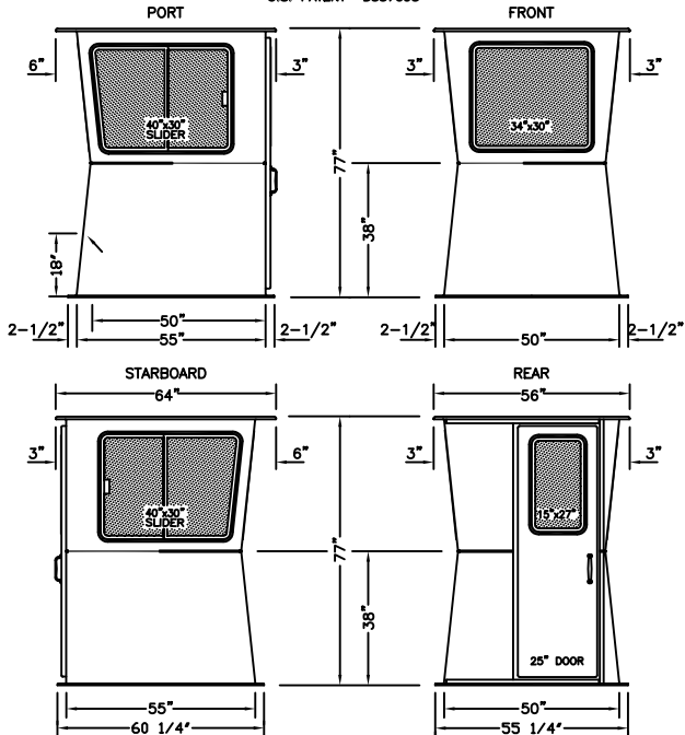
MODEL 2P-6 TWO PERSON PILOTHOUSE WITH REAR SLIDING DOOR 400 LBS. U.S. PATENT D337093
