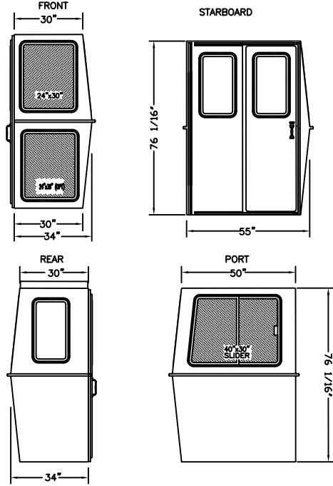
MODEL C-2 ONE PERSON PILOTHOUSE WITH STBD SLIDING DOOR 300 LBS. U.S. PATENT D337093
