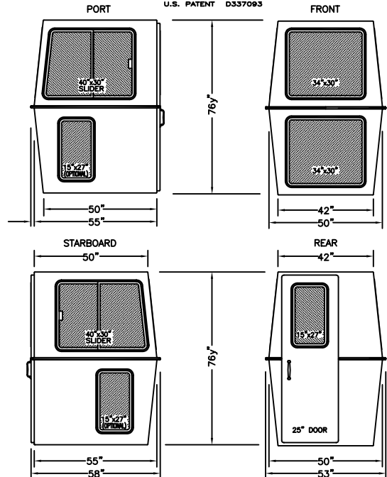
MODEL 2C-1 TWO PERSON CAB WITH INTEGRAL FLOOR AND REAR HINGED DOOR 350 LBS. U.S. PATENT D337093
